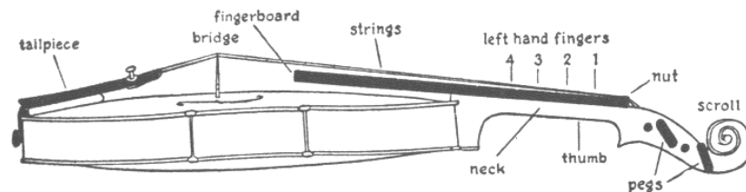
Fig. 2. Violin
