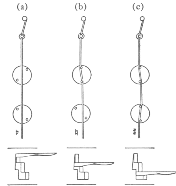
Fig. 106. Pedal Action of the Harp
