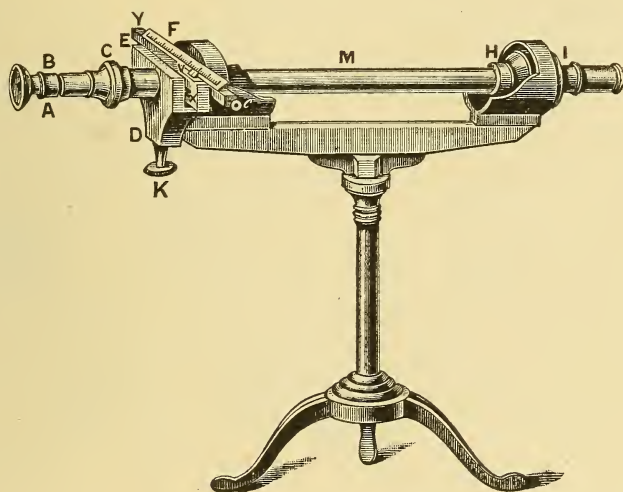
Soleil-Ventzke's saccharimeter.
