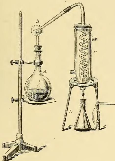
Kjeldahl's nitrogen apparatus. (Simon.)
