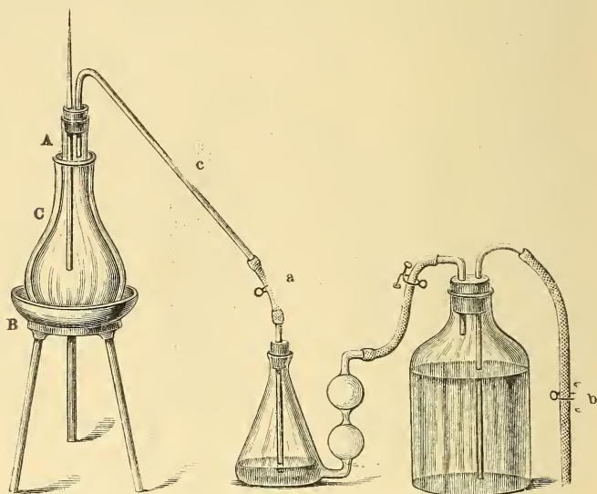
Apparatus for the determination of nitrogen. (Simon.)
